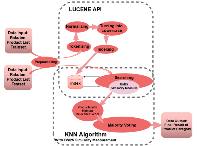
Figure 1: A KNN+BM25 Classifier System
