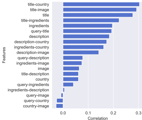
Figure 3: This figure shows the calculated correlation between interaction terms and the click labels. Larger values indicate closer connections.
