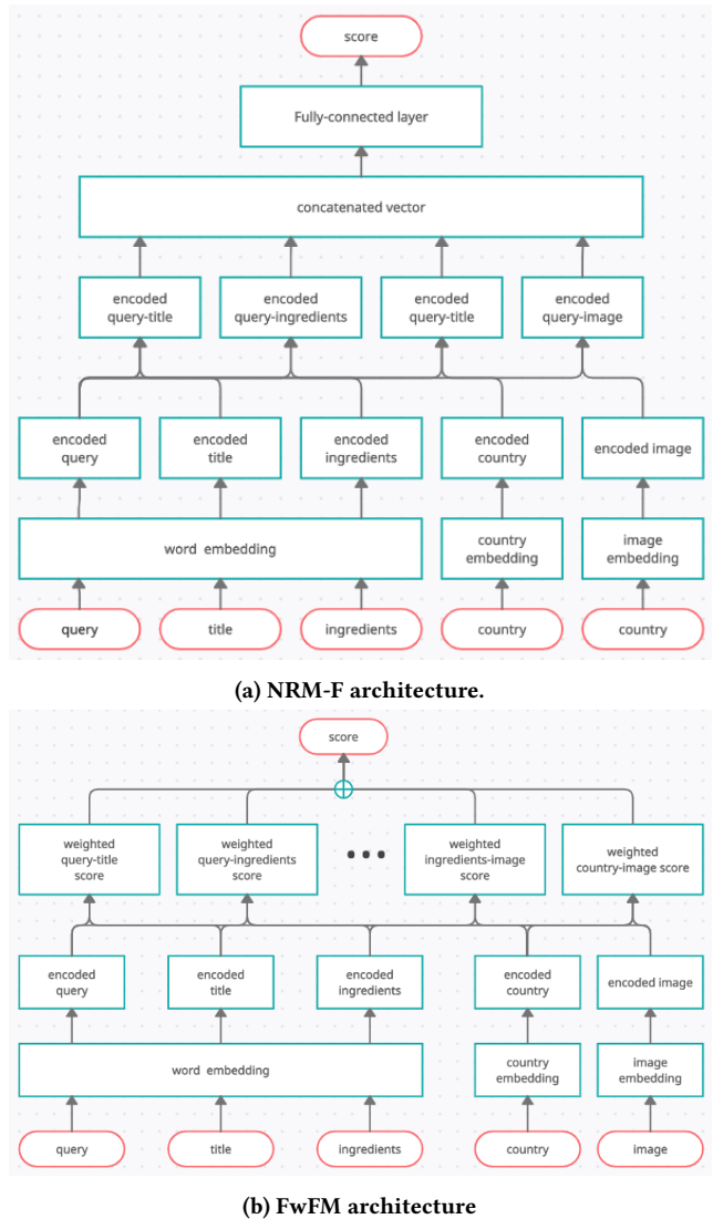
Figure 1: Architecture of field-aware models considered.
